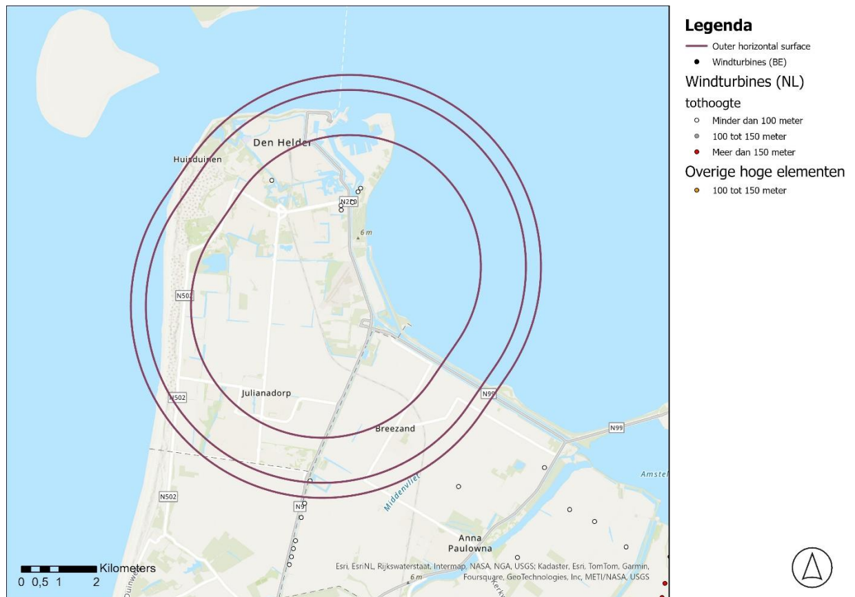
figuur 3-17: Outer horizontal surface De Kooy
