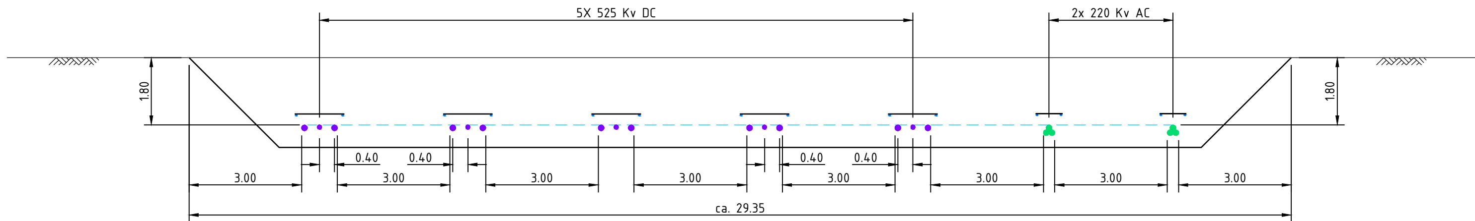
CROSS SECTION 1 – 10.7 GW; OPEN EXCAVATION
