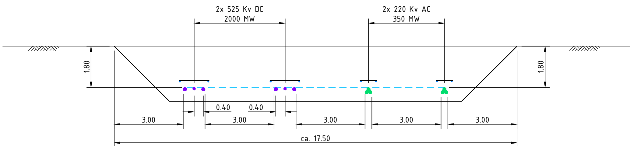
CROSS SECTION 1 – 4.7 GW; OPEN EXCAVATION
