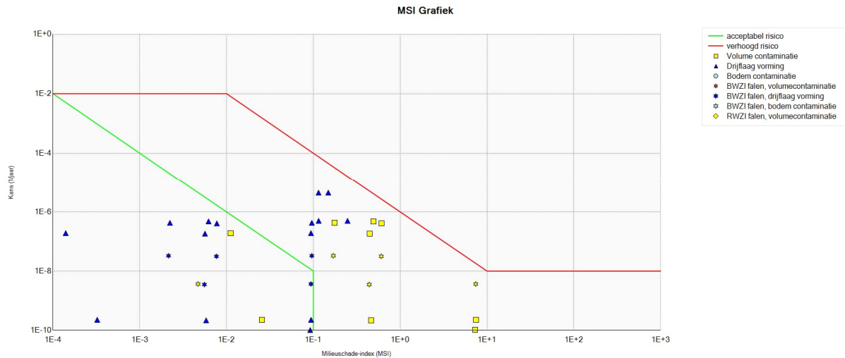
Figuur 5.20. Tank 907 (treated feedstock 6000m 3 ).
