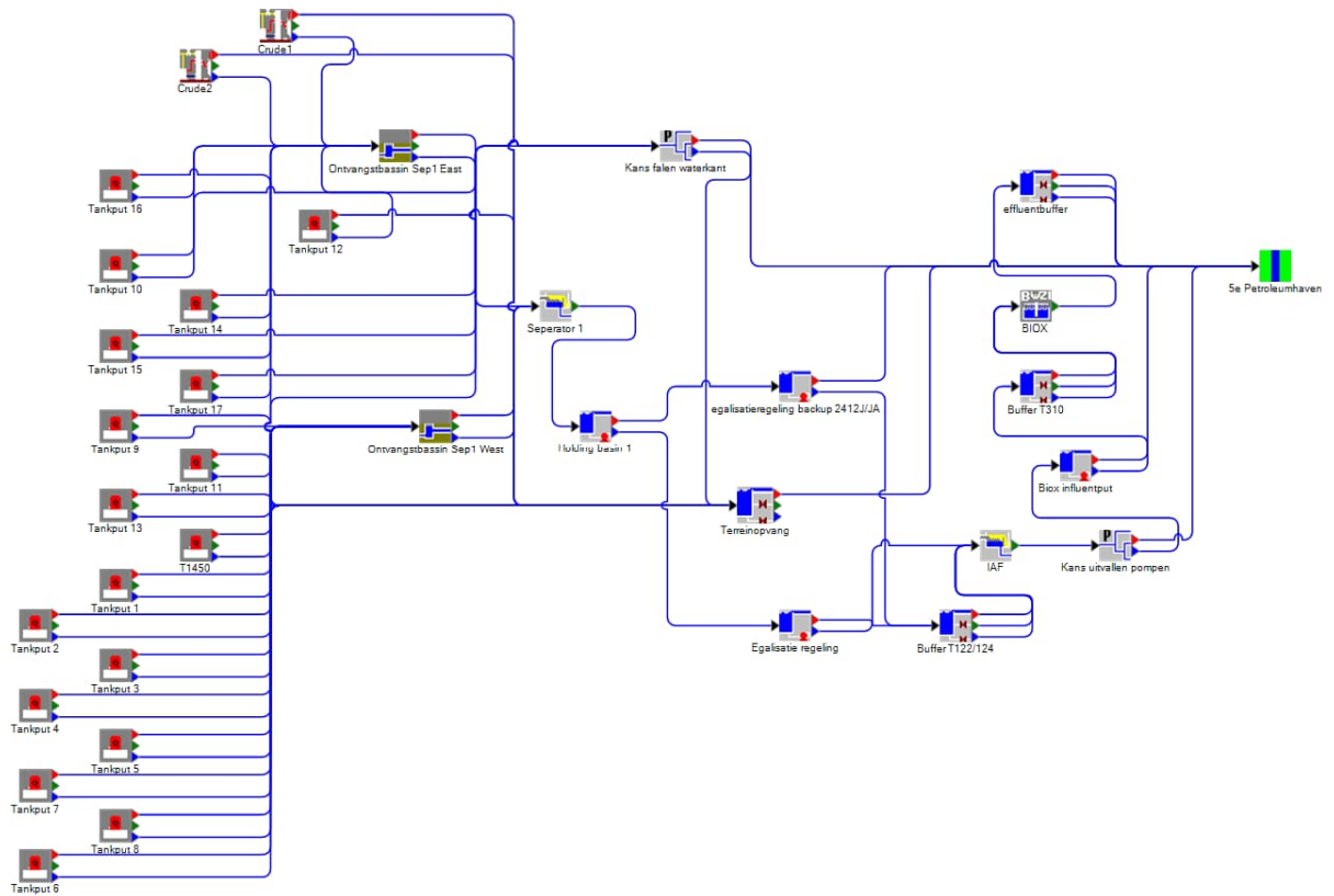
Figuur 4.5: Lozingspad separator 1 (west/east) via IAF/BIOX.
