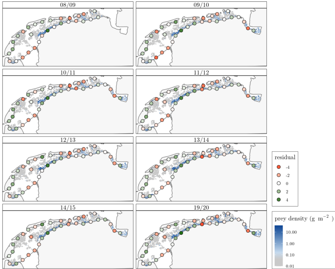
Figure 104: Residuals between the observed and implied number of Avocets at the virtual roosts.
