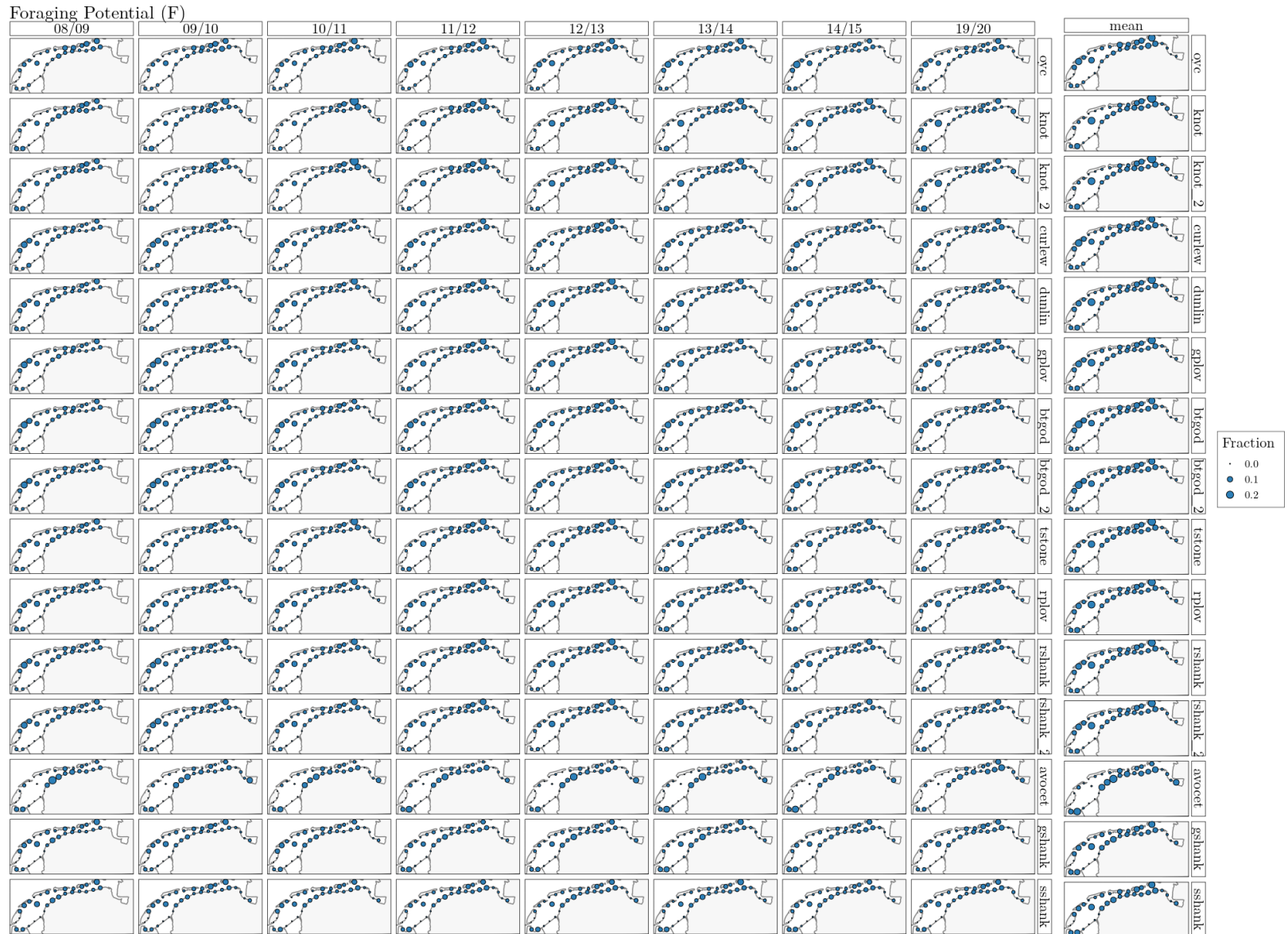
Figure 118: Relative foraging potential along the virtual roosts. Foraging potential is the weighed biomass at the virtual roost, i.e. P_{js} (eqn.1). When in the right margin “_2” is added to the shorebird species, it refers to the second period as defined in section 2.3.
